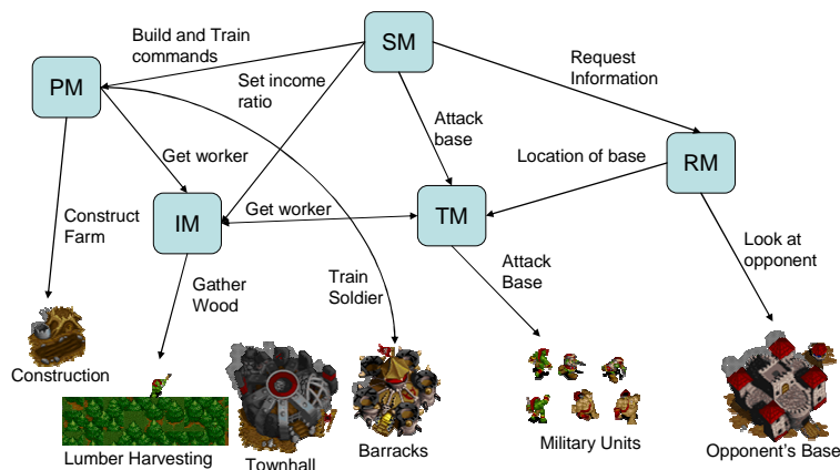
Figure 1 - This graph shows a small sample of the dependencies managers have on one another. The blue boxes are managers with abbreviated names (TM is tactics manager, RM is recon manager, etc). At the bottom of the graph are game entities found in Wargus.
